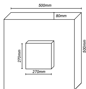
Ref. 10106 Soquete 4 x E27 C L A 480 x 480 x 80 mm
